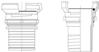
Multi-serrated tail
